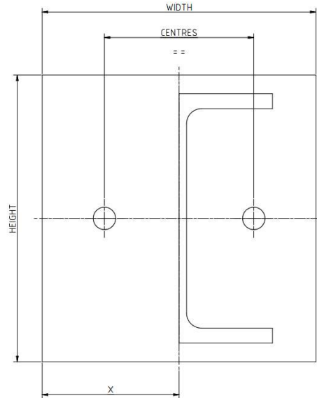
PFC END PLATE TYPE 2
