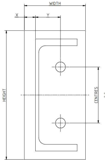
PFC END PLATE TYPE 1
